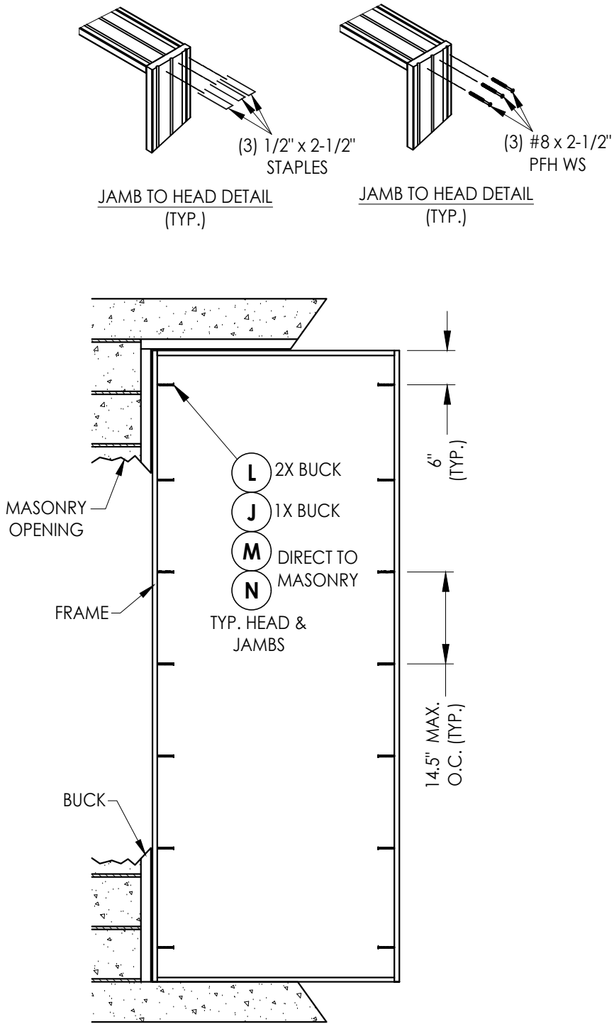
FRAME ANCHORING
