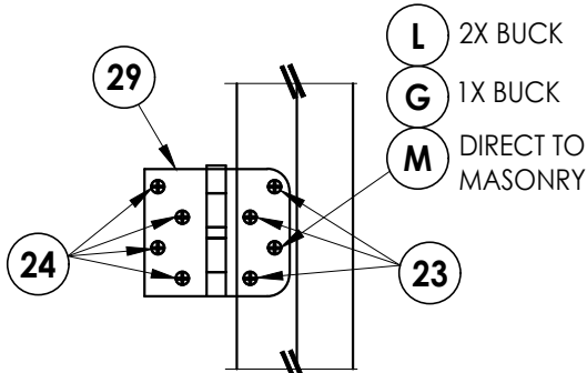
HINGE DETAIL
